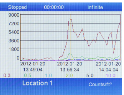
Profile of 0.3 to 10 \mu\text{m} particles captured over 15 minutes window.
